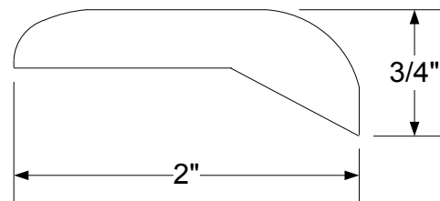
Large Carpet Binder
