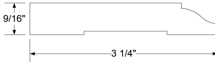
Base
