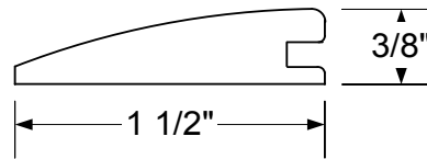
3/8" Reducer
