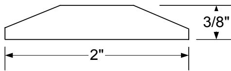
Medium Saddle
