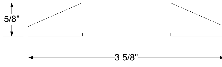
Saddle
